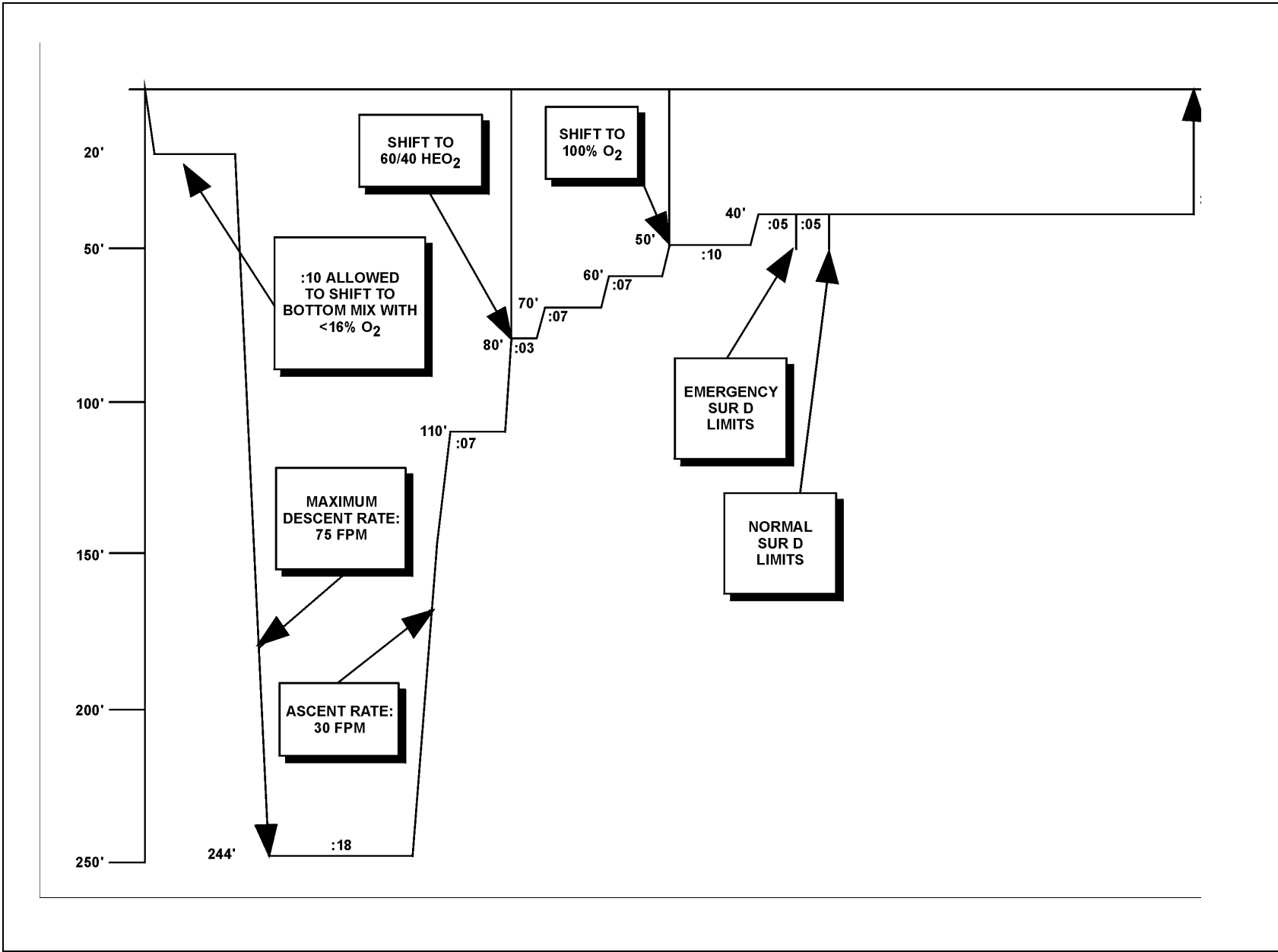
Figure 14-2. In-Water Decompression Dive Profile for a 249 fsw/:18 Dive.
